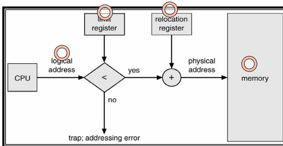
Contiguous Allocation
