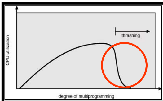
Thrashing
