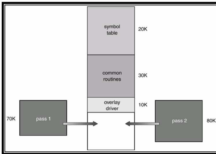
Overlays Example
